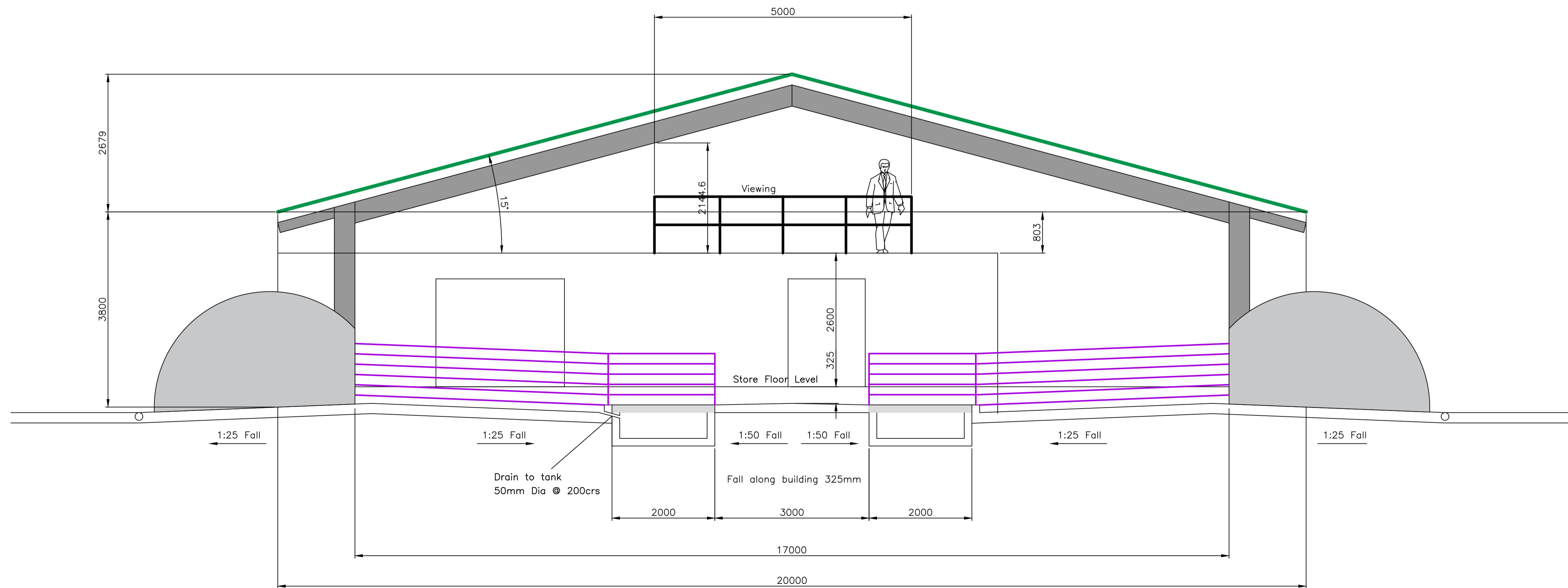
Section B-B
